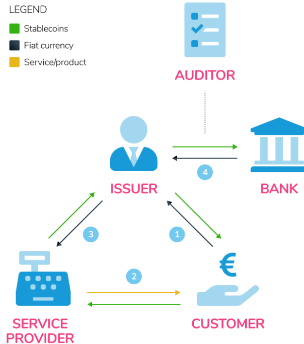
Figure 2: A flow of fiat money and stablecoins in a closed loop SCaaS ecosystem.
